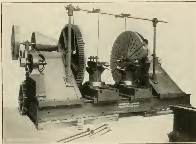
SELLERS' WHEEL LATHE.
